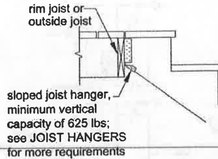
Figure 31. Stair Stringer Attachment Detail.
