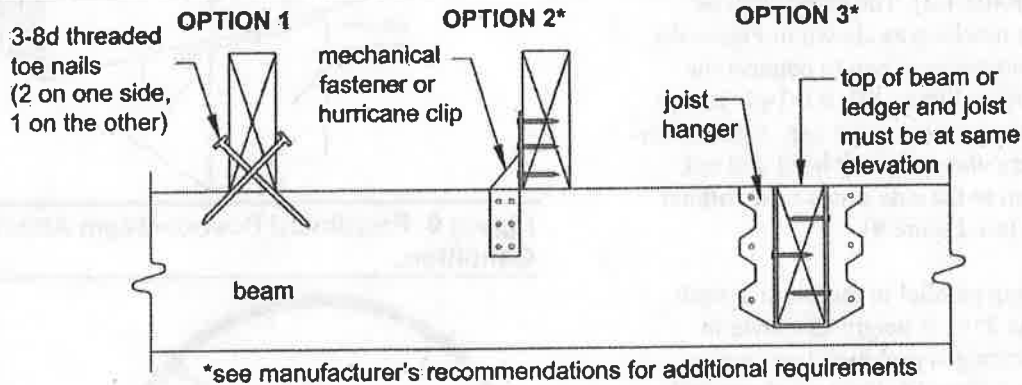
Figure 6. Joist-to-Beam Detail.
